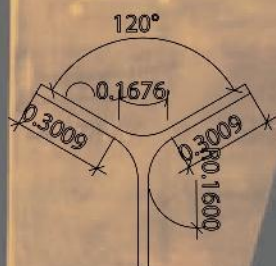
Code: Big Size-Arc Star-3535 / Puzzle light 34 w/m, 4000 lm/m
