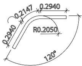
Code: Big Size-Arc 120°-3535 / Puzzle light 23 w/m, 2700 lm/m
