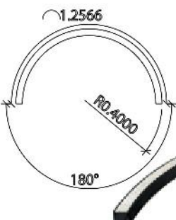
Code: Big Size-C180°R40-3535 / Puzzle light 36 w/m, 4300 lm/m
