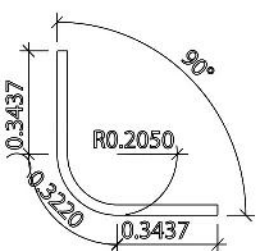
Code: Big Size-Arc 90°-3535 / Puzzle light 30 w/m, 3500 lm/m
